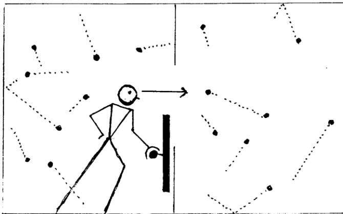
Figure 1. The demon van Maxwell (after Bennett, 1987)
