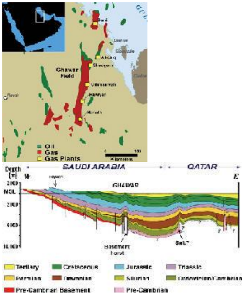
Figure 11. The Ghawar Oil Field (Saudi Arabia) by far the largest conventional oil field in the world. Geologically you need five conditions to form a large oil accumulation, and these things came together in a beautiful manner over a very large area in the Ghawar area. It starts to decline in production at an alarming rate.
